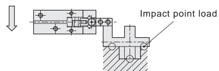
✗ Incorrect claw piece (attached fixture) impact
