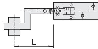
✗ Incorrect (too long holding point)
